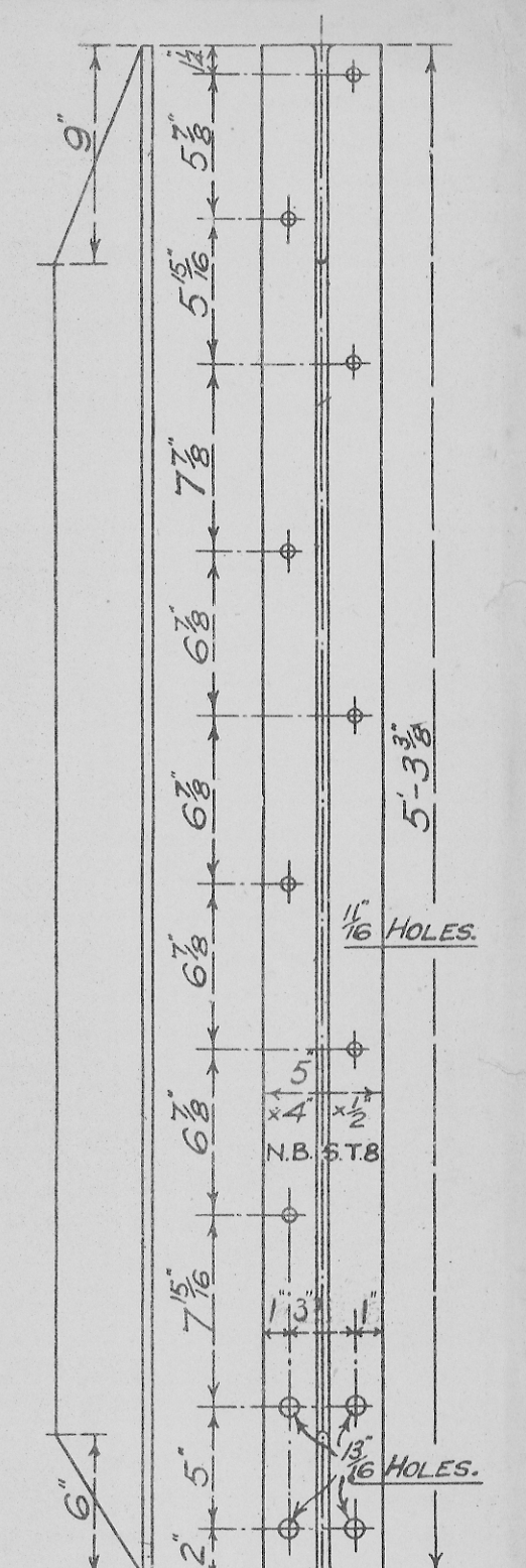
WASHER PLATES TO CORNER PLATE 4 PER SET 'A' 4 PER SET 'B'
