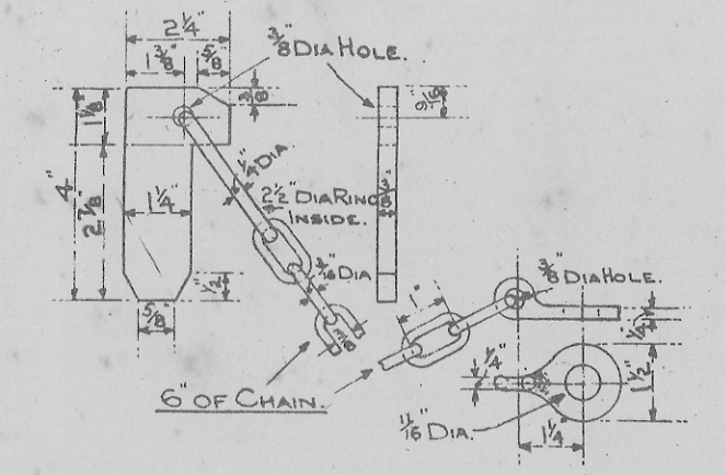
DETAIL OF COTTER & CHAIN 9.
