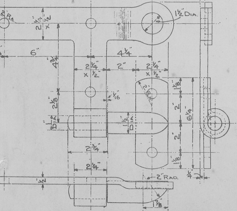
DETAIL OF ITEMS 1 & 2. R & L.
