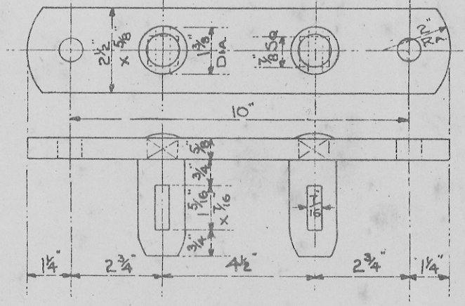
DETAIL OF ITEM 8.
