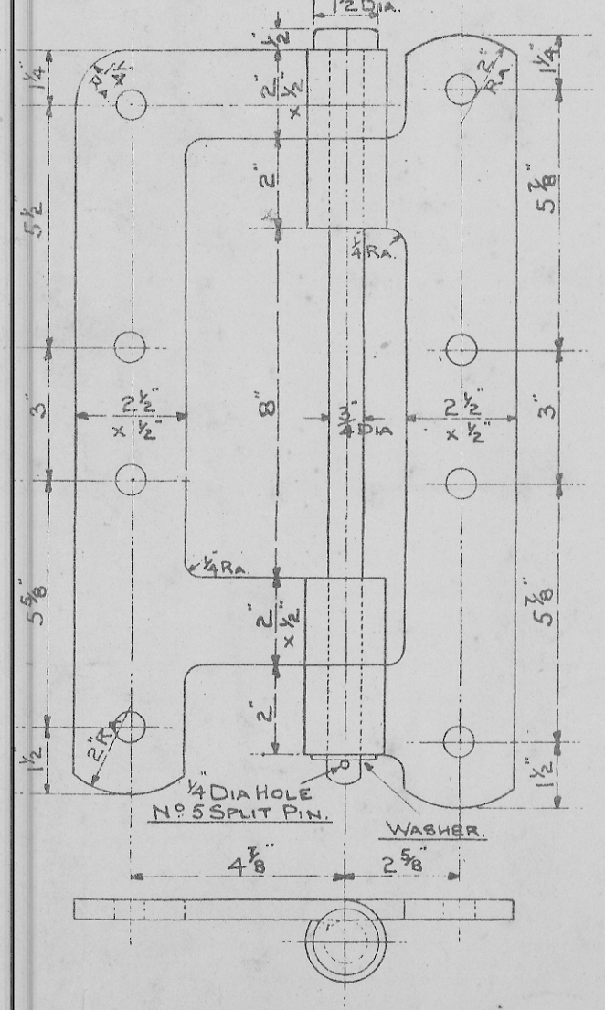
DETAIL OF HINGE 5 & 6 R & L.
