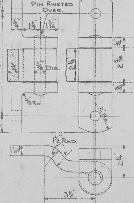
DETAIL OF HINGE 7.
