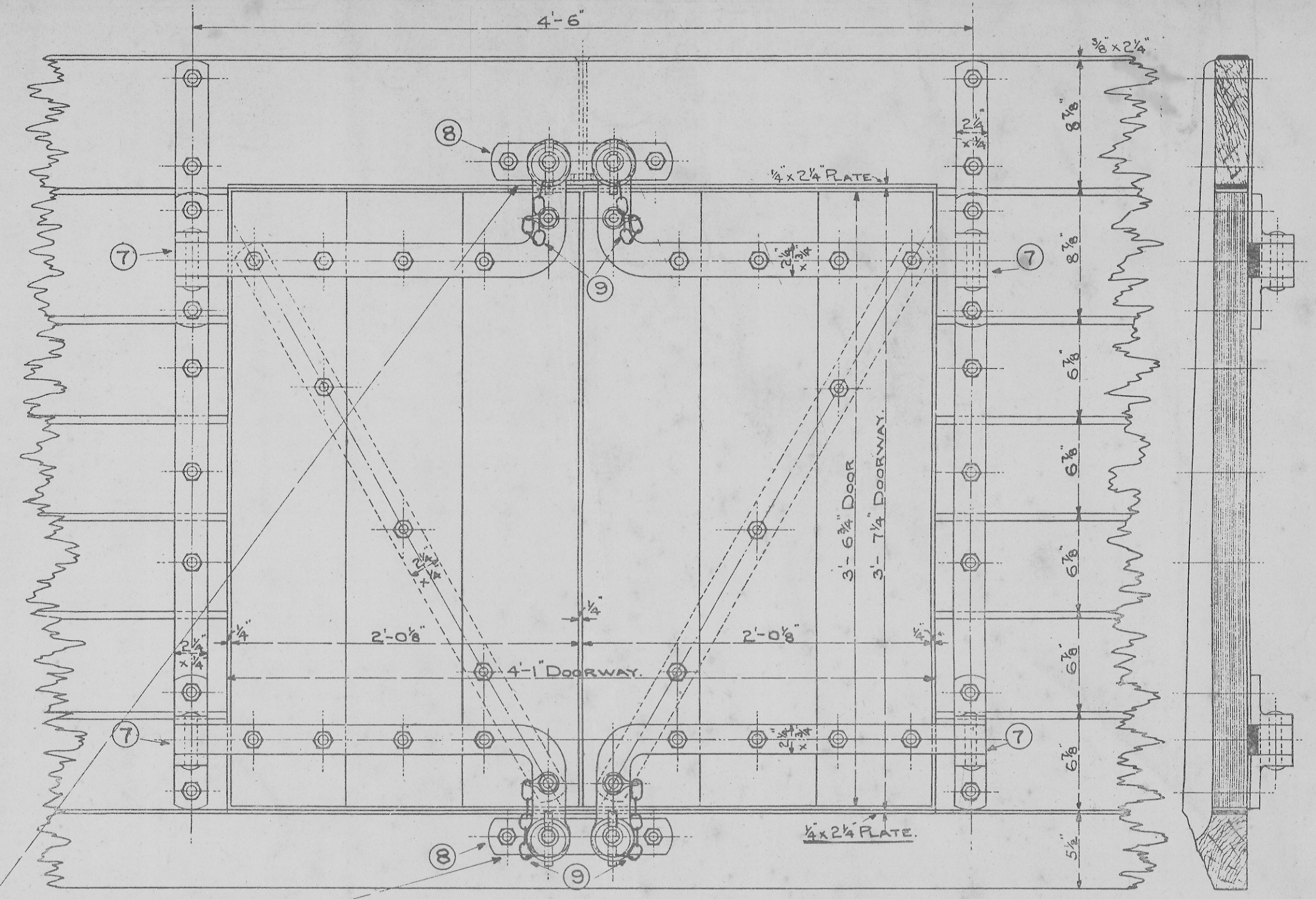
SIDE ELEVATION
