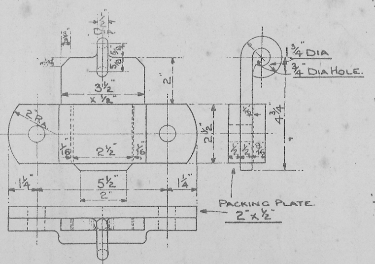
DETAIL OF ITEMS 3 & 4.
