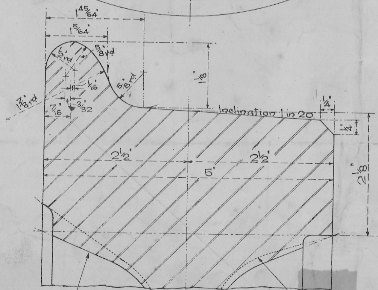
SECTION OF RIM. (All Wheels). Full lines for 20 Ton ordy. & Tanks. — Full Size. — Dotted lines for 12 Ton ordy. & 10, 12 & 14 Ton Tanks.
